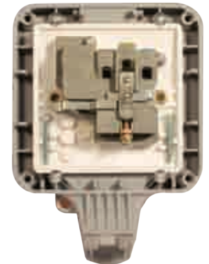
Angled in-line, colour coded, captive terminals
