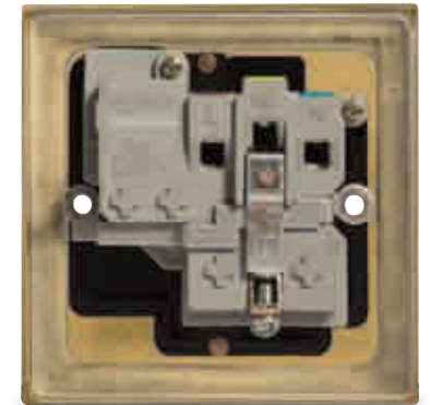
Angled in-line, colour coded, captive terminals
