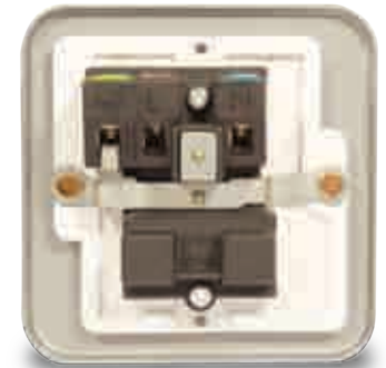
Angled in-line, colour coded, captive terminals
